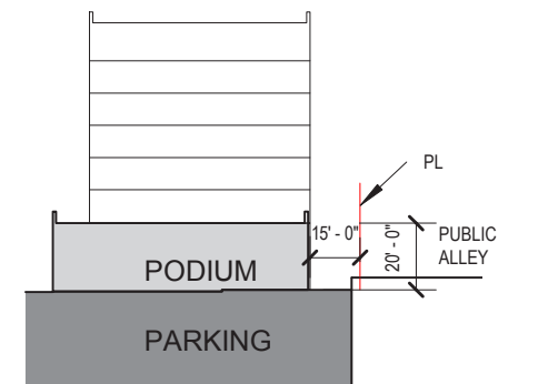
3 REAR YARD SECTION 2 1/64" = 1'-0"
